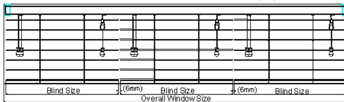
3-on-1 Headrail (IB)
